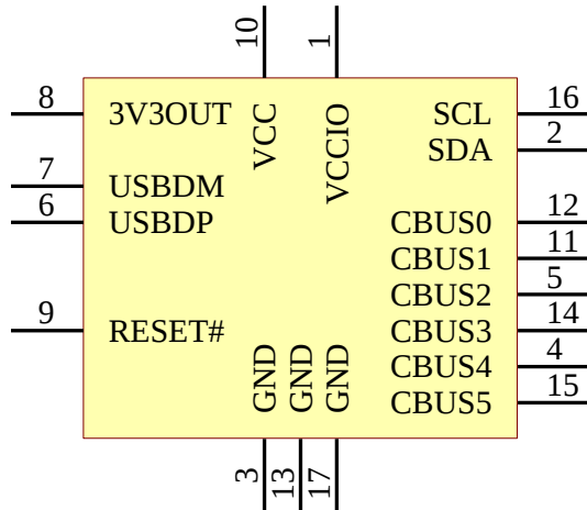
Figure 3.1 QFN Schematic Symbol
