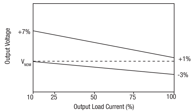
12V Output
