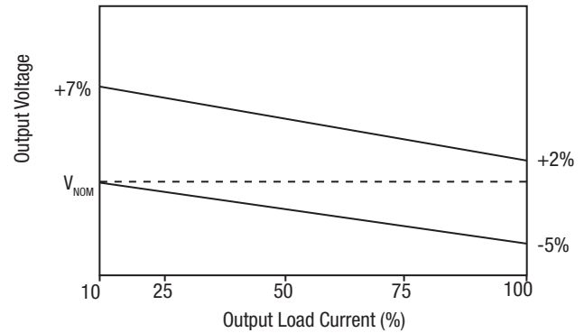
12V Output
