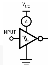
Figure 7. I CCD Test Circuit
