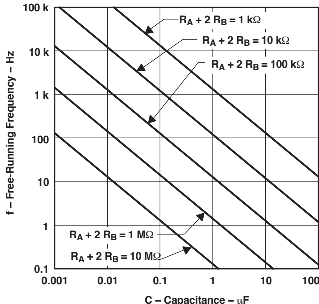
Figure 14. Free-Running Frequency
