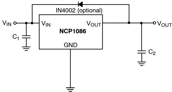
Figure 18. Protection Diode Scheme for Large Output Capacitors (3.3 V Fixed Output)
