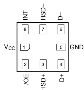
Figure 4. UMLP (Top Through View)
