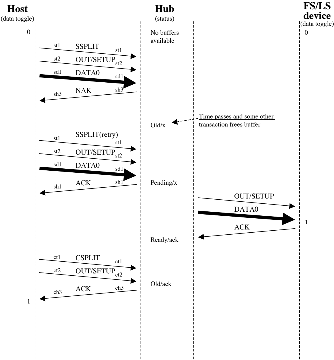
Figure A-15. No buffer Available No Smash (HS NAK(S))
