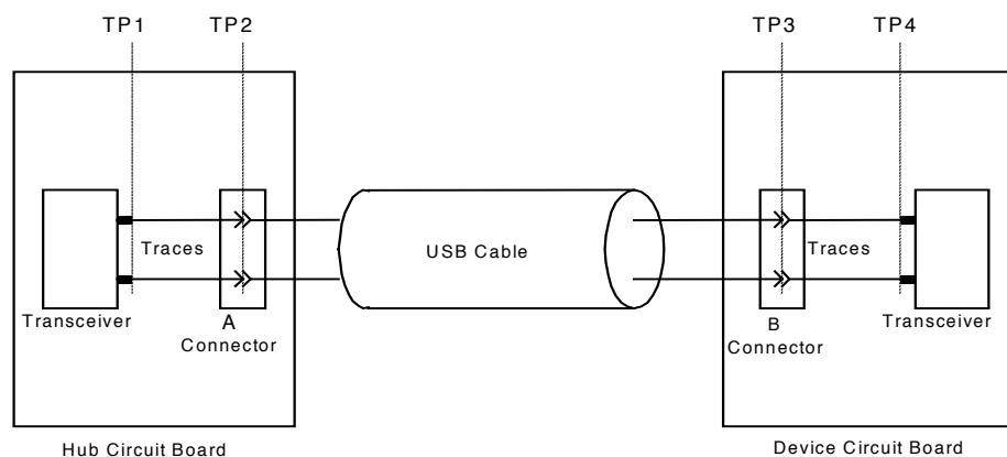
Figure 7-11. Measurement Planes
