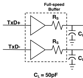
Figure 7-9. Full-speed Load
