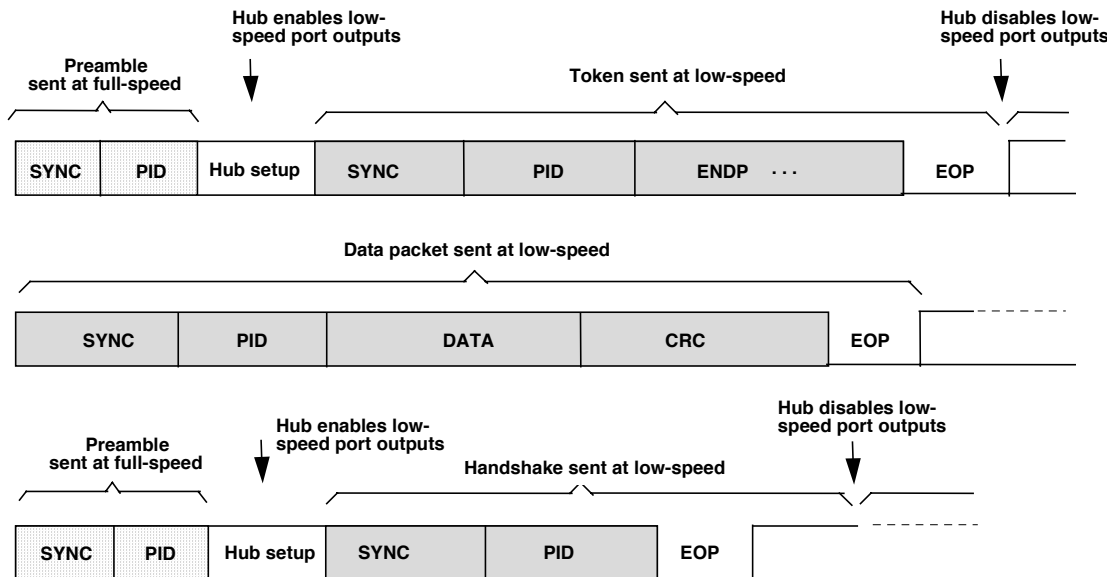
Figure 8-48. Low-speed Transaction
