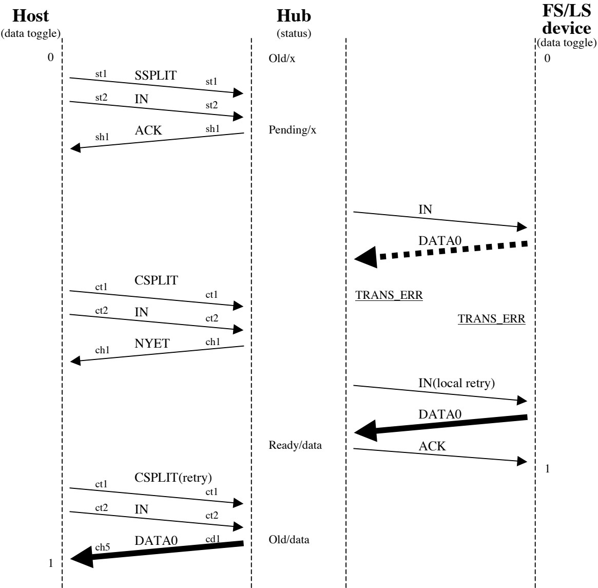
Figure A-36. Normal FS/LS DATA0/1 Smash
