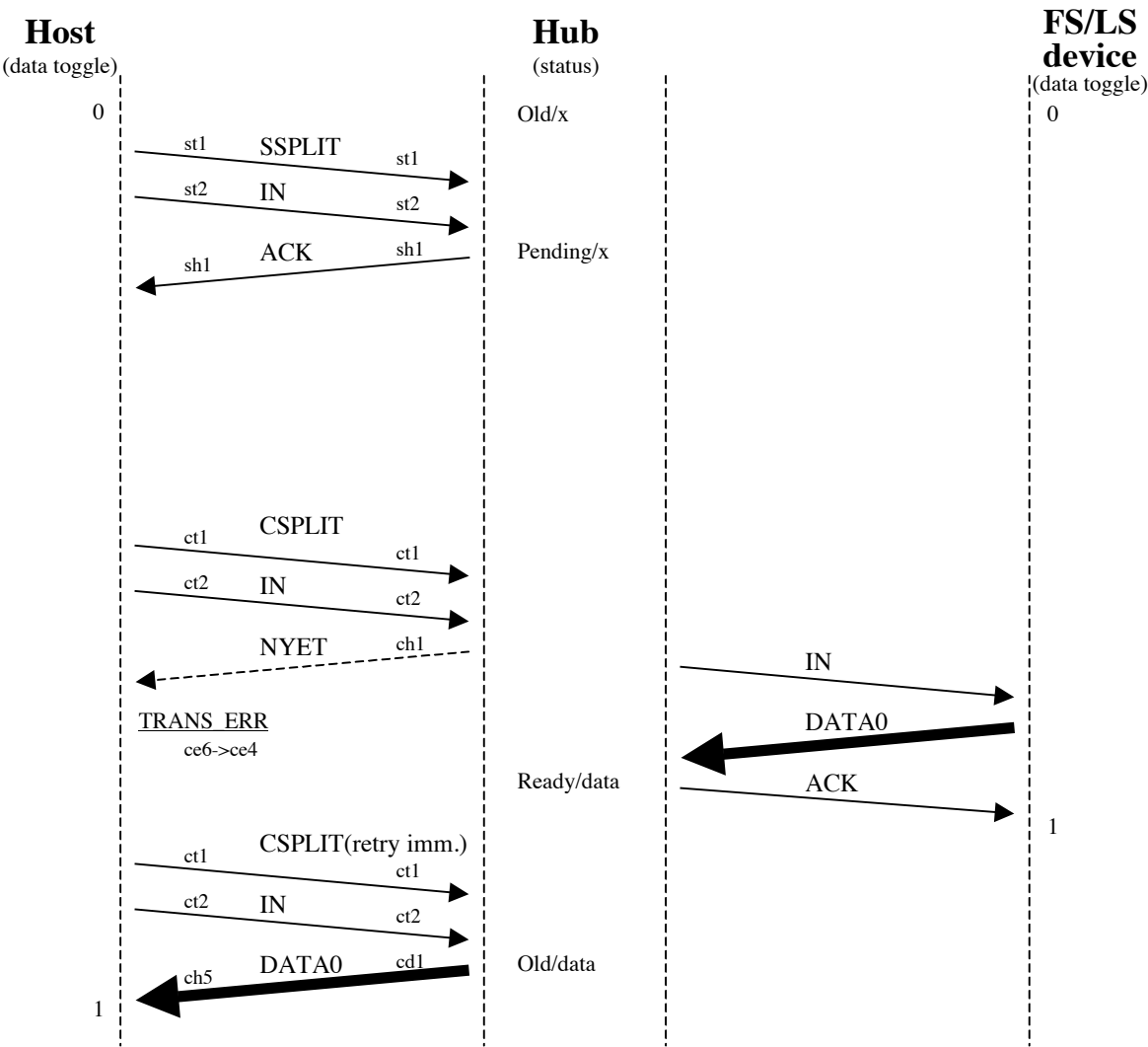
Figure A-43. CS Earlier HS NYET Smash(case 1)
