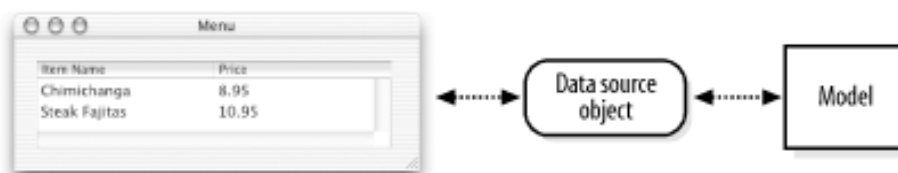
Figure 9-3. A data source as a controller between a model and a view
