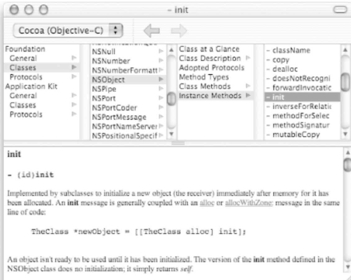
Figure C-3. Using Cocoa Browser to access API reference documentation
