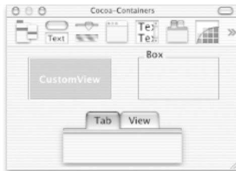
Figure 7-2. Drag a CustomView object from the Cocoa-Containers window into the project window
