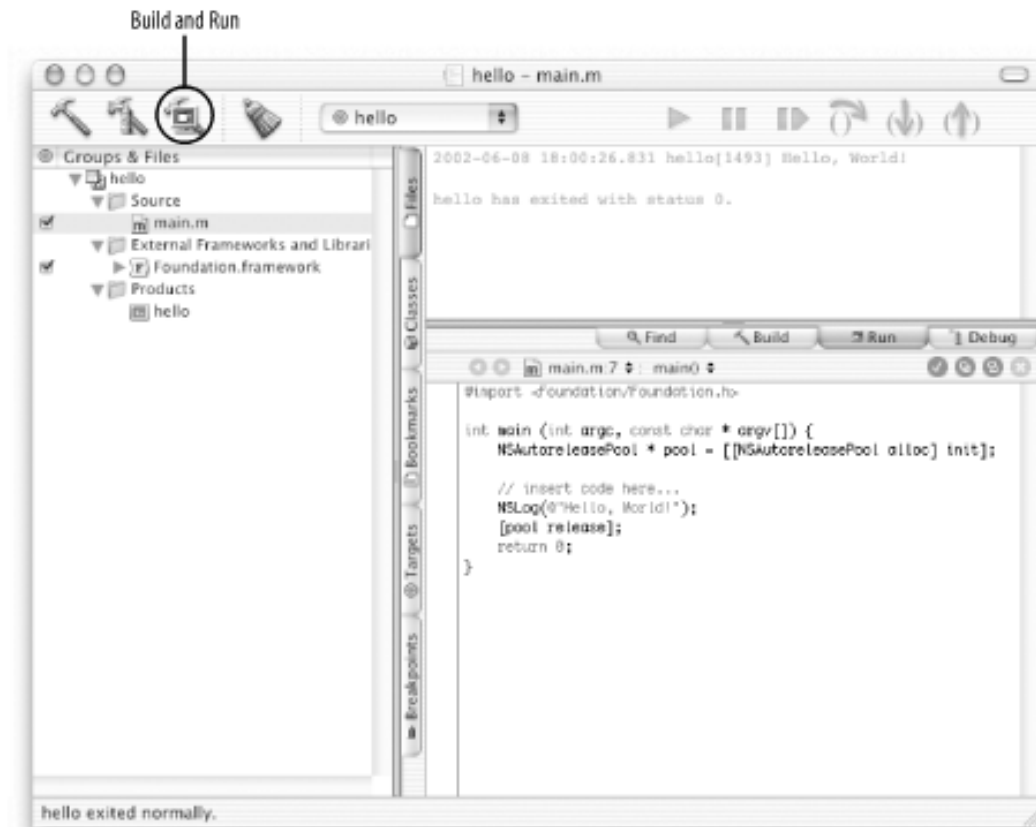
Figure 2-10. Project Builder's main window after running Hello World
